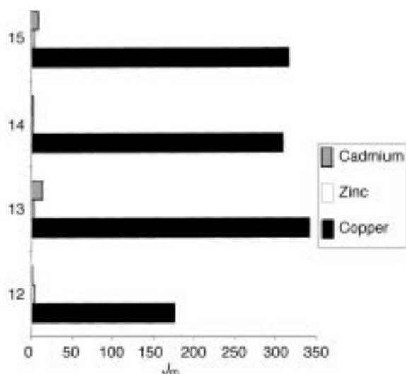
Fig. 1 Transport profile of alkylated benzimidazolecarboxylic acid ligands 12–15 for \text{Cu}^{2+} , \text{Zn}^{2+} and \text{Cd}^{2+} from multiple-ion transport experiments. Feed phase; [\text{M}^{2+}]_{\text{total}} = 0.3 \text{ mol dm}^{-3} , pH 5.05, \text{NaO}_2\text{CMe} buffer. Bars represent J_m (moles transported 24 h) \times 10^7
